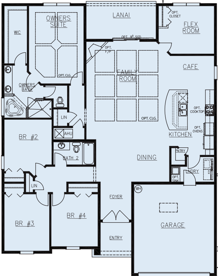
FLOOR PLAN
